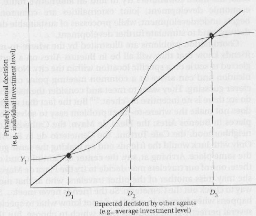
Figure 5.1 Multiple Equilibria
