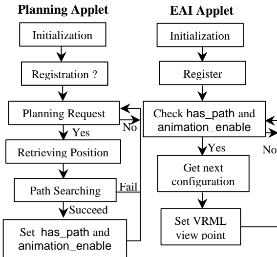
Figure 4: Flow charts for the main loops of the planning and EAI applets
