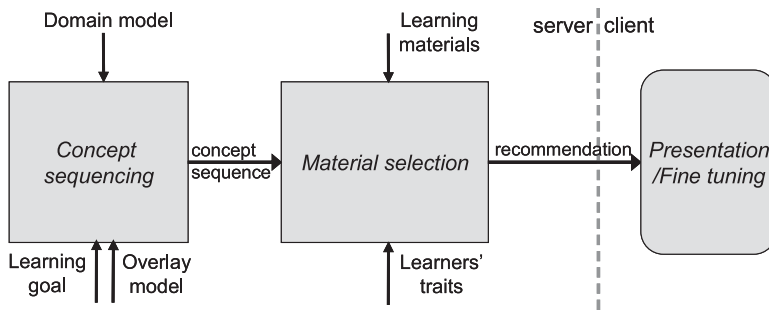
Fig. 3. The flow of adaptivity in CooTutor.
