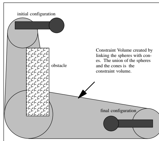
Figure 4. Constraint Volume specified by placing a set of circles (spheres for 3d) of various sizes.
