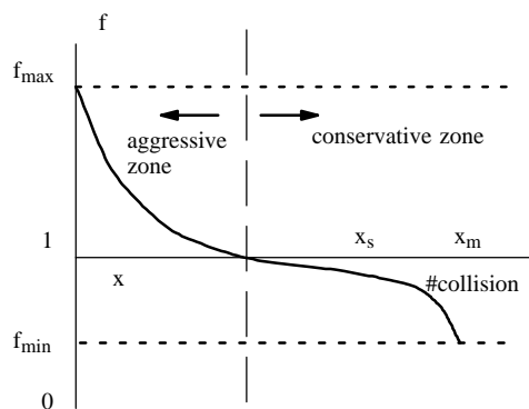
Figure 3. Search resolution refinement model: collision ratio dependent step size. Note x_m = 728 for 6 dof.
