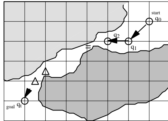
Figure 1. Search resolution in C-space. The circled configurations are attainable at the grid resolution. The triangle ones are attainable at half that resolution. The = signed one is available at one third of the initial resolution. Here the moving object is a point.
