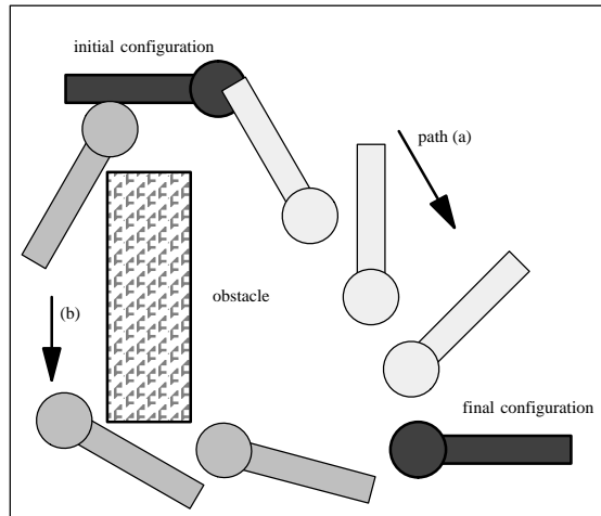
Figure 2. Typical potential guided planner will find (a) before (b), because (a) is shorter.
