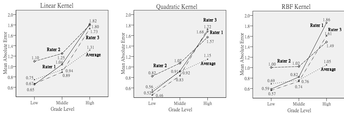
Figure 3. Mean absolute error of the three raters and the average trained models at three grade levels.
