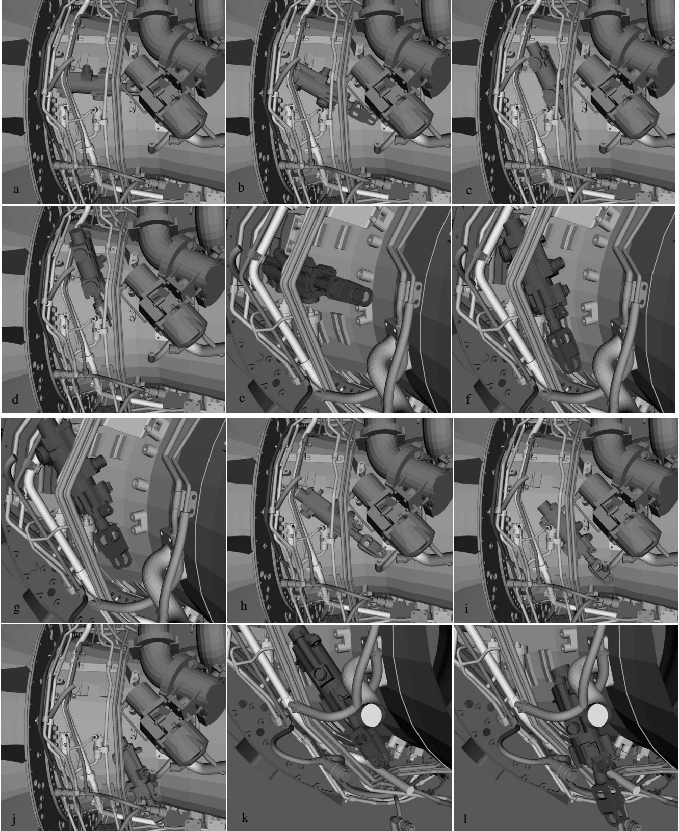
Figure 8. The effect of constraint volume. (a) through (d) shows the LRU being accessed through the designed opening. (e) through (g) show some close ups. Another path was shown in (h) through (j) with two close ups in (k) and (l).
